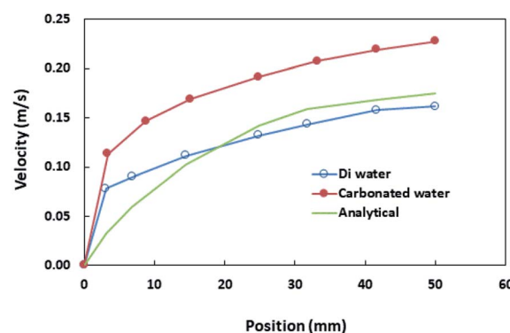
Fig. 3 The translational velocity of distilled and carbonated water droplets. The droplet volume is 40 \mu L and the inclination angle of the surface ( \delta ) is 5°. The analytical solution predicted from eqn (5) is also shown for comparison.
