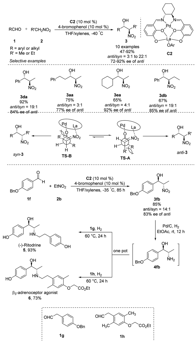
Scheme 4 Catalytic asymmetric anti -selective Henry reactions with Nd/Na/L1 heterobimetallic complex.
