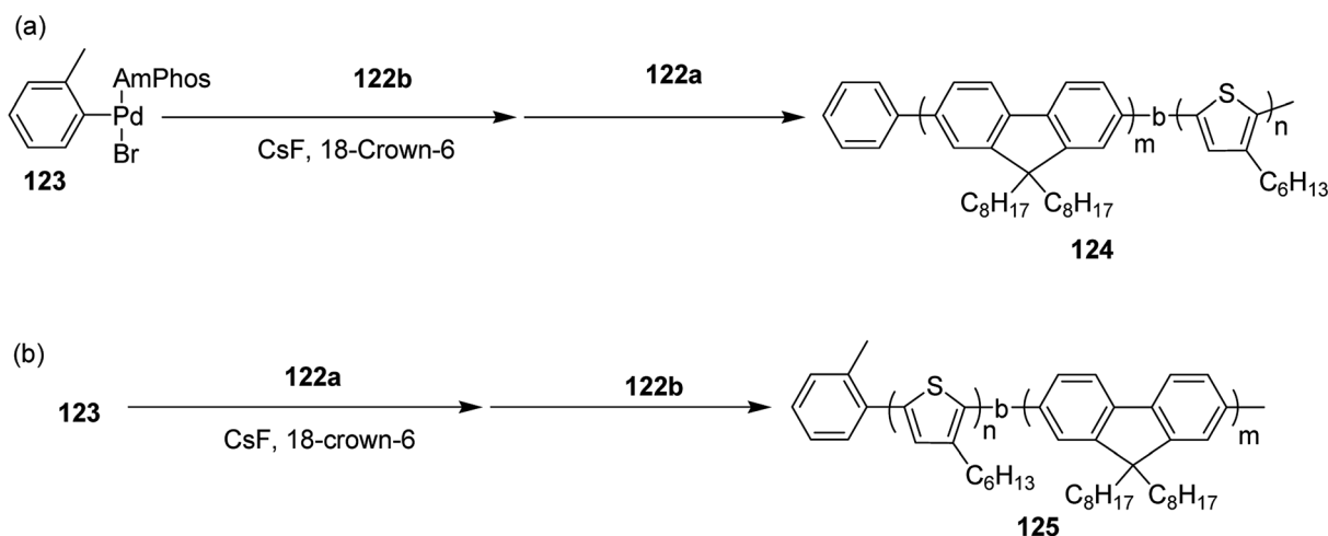
Scheme 39 Block copolymerization of 122a and 122b with Pd initiator 121 at room temperature to synthesize copolymers 124 and 125 .
