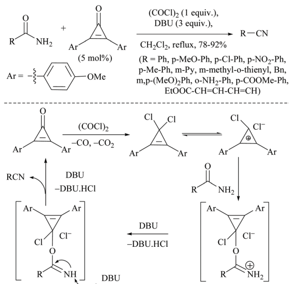
Scheme 52 Organocatalytic dehydration.
