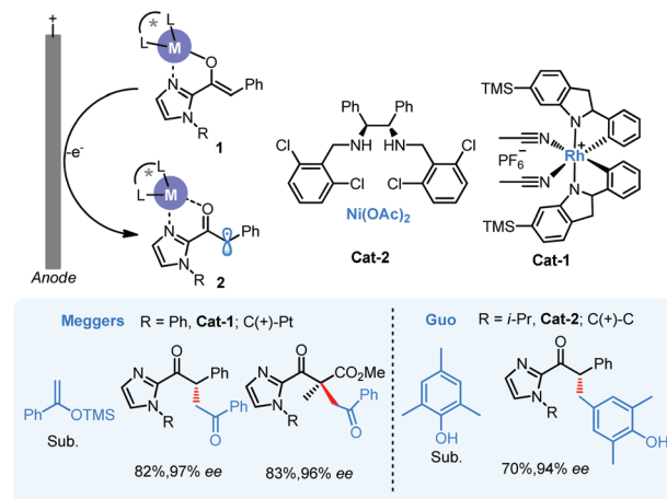
Scheme 2 Asymmetric electrochemical catalysis with α-carbonyl radicals 2 .
