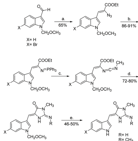
Scheme 30 Iminophosphorane-mediated ring formation to produce (Z)-aplysinsin derivatives. Reagents: (a) \text{N}_3\text{CH}_2\text{COOC}_2\text{H}_5 , NaOEt, EtOH, -15\text{ }^\circ\text{C} , (b) \text{PPh}_3 , \text{CH}_2\text{Cl}_2 , rt, (c) \text{CH}_3\text{-NCO} , toluene, rt, (d) \text{NH}_2\text{R} , toluene, 45\text{ }^\circ\text{C} , (e) \text{HCOOH} , reflux.
