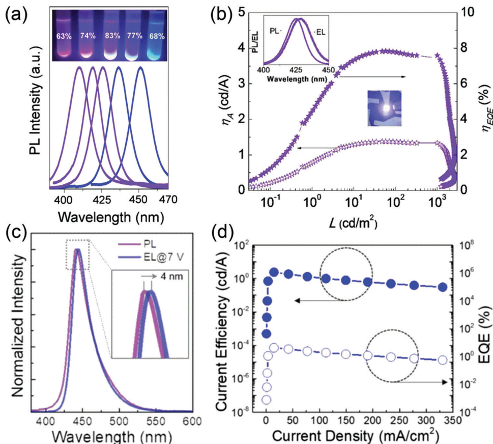
Fig. 11 (a) Normalized PL spectra of ZnSe/ZnS core/shell QDs (dispersed in hexane) under the radiation of an ultraviolet lamp. (b) Current efficiency- \eta_{\text{EQE}} - L characteristics for the ZnSe/ZnS-based QD-LEDs. Reproduced with permission. 98 Copyright 2015, Royal Society of Chemistry. (c) Spectral comparison of the PL of a dilute ZnSeTe/ZnSe/ZnS QD dispersion with the EL collected at 7 V. (d) Current efficiency and \eta_{\text{EQE}} as a function of current density for QD-LEDs with an ITO/PEDOT:PSS/PVK/ZnSeTe/ZnSe/ZnS QDs/ZnMgO/Al structure. Reproduced with permission. 102 Copyright 2019, American Chemical Society.
