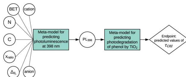
Fig. 2 Determination of photodegradation of phenol by titanium dioxide ( \tau_{OH} ) in line with the SAPNet methodology (BET – Brunauer–Emmett–Teller surface area analysis; N, C – the amount of nitrogen and carbon atoms; x_{ratio} – molar ratio (IL : TiO 2 precursor); \Delta_{IL} – decomposition of the ionic liquid during the solvothermal reaction; cation – the type of cation in the IL; anion – type of anion in IL; PL 398 – the intensity of the photoluminescence signal at 398 nm).
