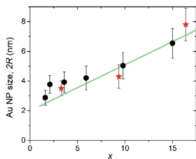
Fig. 7 Dependence of the Au NP size ( 2R , here R is the spherical NP radius) on the Au concentration ( x ) in the \text{Au}_x\text{C}_{60} mixture films as obtained from the TEM analysis (red stars) and from the Scherrer analysis of the XRD line-broadening (black circles).
