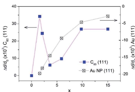
Fig. 8 The relative change of lattice parameter in fcc- \text{C}_{60} (blue boxes) and in fcc-Au NPs (crossed circles) upon increase of Au concentration x in the \text{Au}_x\text{C}_{60} mixture films.
