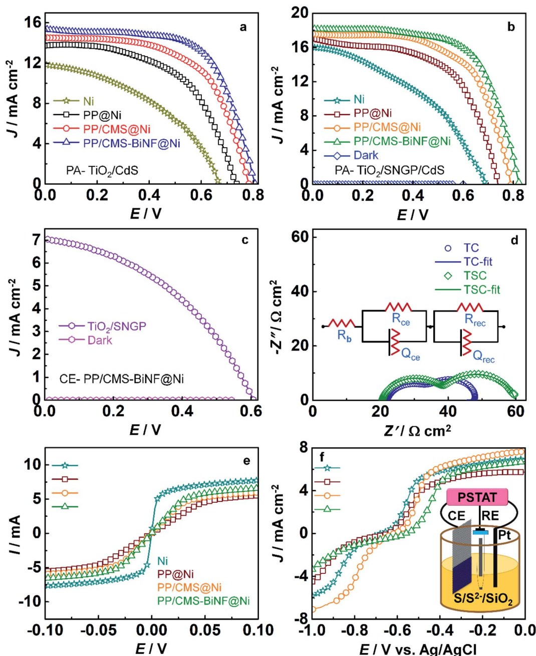
Fig. 4 J–V plots of solar cells with (a) \text{TiO}_2/\text{CdS} and (b) \text{TiO}_2/\text{SNGP}/\text{CdS} photoanodes with four different CE: Ni foam, PProDOT@Ni foam, PProDOT/CMS@Ni foam and PProDOT/CMS-BiNF@Ni foam in a polysulfide/silica gel electrolyte under 1 sun illumination and in the dark. (c) J–V plots of a \text{TiO}_2/\text{SNGP}-\text{S}/\text{S}^{2-}/\text{silica gel}-\text{PProDOT}/\text{CMS}-\text{BiNF@Ni} foam cell under 1 sun illumination and in the dark. (d) EIS spectra of \text{TiO}_2/\text{CdS} (TC) and \text{TiO}_2/\text{SNGP}/\text{CdS} (TSC) photoanodes in a \text{S}/\text{S}^{2-}/\text{silica gel} and PProDOT/CMS-BiNF@Ni foam in the dark. (e) I–V plots of Ni foam, PProDOT@Ni foam, PProDOT/CMS@Ni foam and PProDOT/CMS-BiNF@Ni foam in a three-electrode system using \text{S}/\text{S}^{2-}/\text{silica gel} electrolyte. (PP: PProDOT, CMS: carbon micro-spheres, BiNF: Bi nanoflakes).
