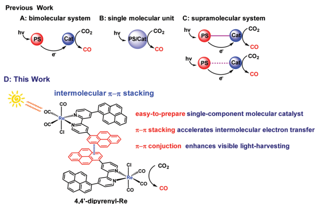
Scheme 1 Strategies for the design of catalysts for photochemical \text{CO}_2\text{RR} .
