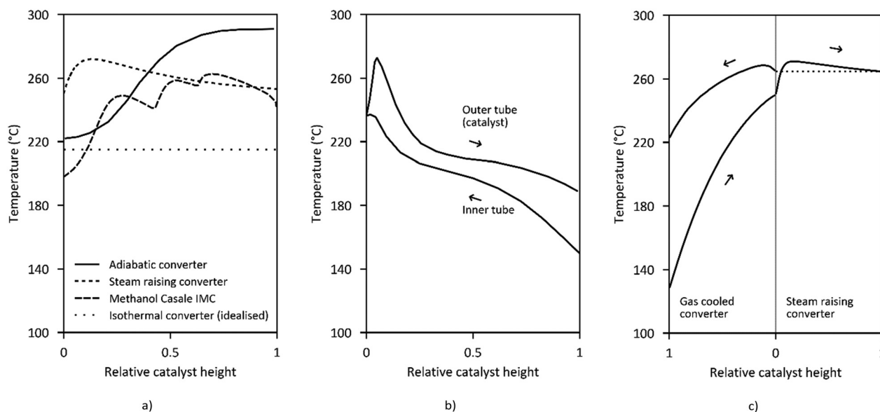
Fig. 7 Temperature profiles along the reactor length of (a) adiabatic converter, 105 steam raising converter, 126 Methanol Casale IMC, 142 and idealized isothermal converter (idealized), (b) Mitsubishi Superconverter, 143 (c) Lurgi MegaMethanol. 99
