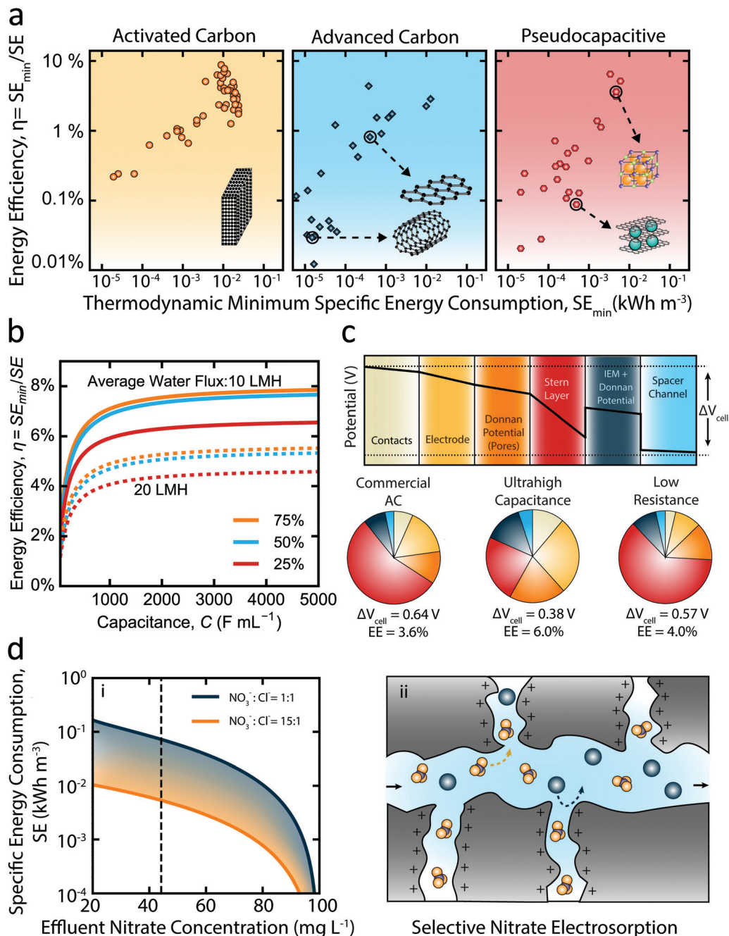
Fig. 4 The effect of enhanced capacitance, resistance, and ion-ion selectivity on the energy consumption of electroremoval. (a) Energy efficiency of capacitive deionization (CDI) versus the thermodynamic minimum specific energy of separation. The data is collected from the literature for (i) activated carbon materials, (ii) advanced carbon materials, and (iii) pseudocapacitive materials. The specific conditions for each data point are listed in Table S1 (ESI†). (b) Modeled energy efficiency of CDI over a range of capacitance values for salt rejections of 25% (red curves), 50% (blue curves), and 75% (orange curves). The feed salinity is 2000 \text{ mg L}^{-1} and the water recovery is 50%. The solid and dashed lines represent average water fluxes of 10 \text{ L m}^{-2} \text{ h}^{-1} and 20 \text{ L m}^{-2} \text{ h}^{-1} , respectively. Additional modeling parameters used are provided in the ESI†. (c) The contribution of each potential drop to the average total cell potential ( \Delta V_{\text{cell}} ) for three materials: commercial activated carbon, theoretical ultra-high capacitance EDL material, and theoretical low resistance EDL material. The potential drop profile shown is for commercial activated carbon and the colors displayed correspond to those used in the charts. The data shown is for 50% salt rejection and 50% water recovery of a 2000 \text{ mg L}^{-1} salinity feedwater. The average water flux is fixed at 10 \text{ L m}^{-2} \text{ h}^{-1} . (d) Selective removal of nitrate using electroremoval. (i) The specific energy consumption of producing varying levels of nitrate effluent concentration for a feedwater composition of 500 \text{ mg L}^{-1} sodium chloride and 100 \text{ mg L}^{-1} nitrate. The blue and orange lines represent \text{NO}_3^-:\text{Cl}^- selectivity ratios of 1 and 15, respectively. The dashed vertical line corresponds to the US EPA maximum contaminant level of nitrate in drinking water of 45 \text{ mg L}^{-1} (or 10 \text{ mg L}^{-1} as N). (ii) Schematic of selective nitrate electroremoval. Nitrate (orange polyatomic molecules) and chloride (blue spheres) migrate through the macropores. The nitrate molecules are preferentially immobilized in the EDLs of the micropores.
