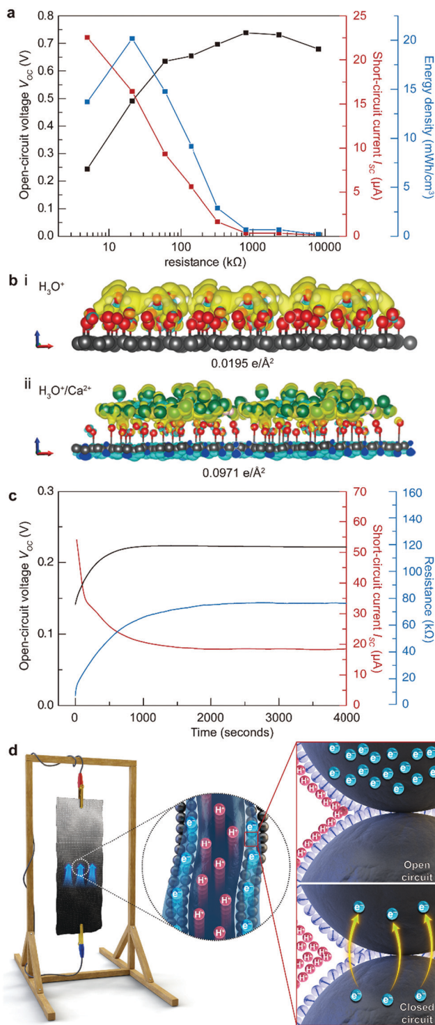
Fig. 4 Effect of resistance and Ca 2+ ions on the energy generation of the STEPG. (a) Measured V_{OC} , I_{SC} and energy density values of various resistance STEPGs at 26 °C and 37% RH. (b) Charge redistribution on oxidized graphene covered by hydronium ions (i) and hydronium ions with calcium ions (ii) (yellow, losing an electron; blue, gaining an electron). The value of the electron redistribution on the carbon is located below each panel. (c) Measured V_{OC} , I_{SC} and resistance profiles after stabilization for 3 hours to reduce the water content and resistance change. (d) Schematic illustration of dielectric scattering on the working STEPG and equivalent electric circuit. Blue balls containing arrows represent water molecules along with their polarity (dielectric field) in the inset.
