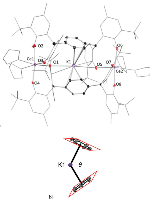
Fig. 2 Solid state structure of complex 2^{Me} . (a) core of anion with K(THF)_7 counter-cation and all H and two lattice THF solvent molecules omitted for clarity. Coordinated solvent shown as wireframe, and ligands shown as capped stick for clarity; thermal ellipsoids of other atoms are shown at 30% probability. (b) Bis( \eta^6 -arene) coordination of the endo K + cation with the angle between the two arene planes labelled as \theta .
