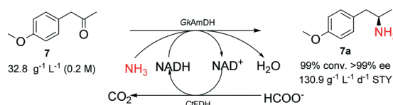
Scheme 3 Synthesis of 4-methoxyamphetamine ( 7a ) catalyzed by the GkAmDH/FDH system on a 100 mL scale.
