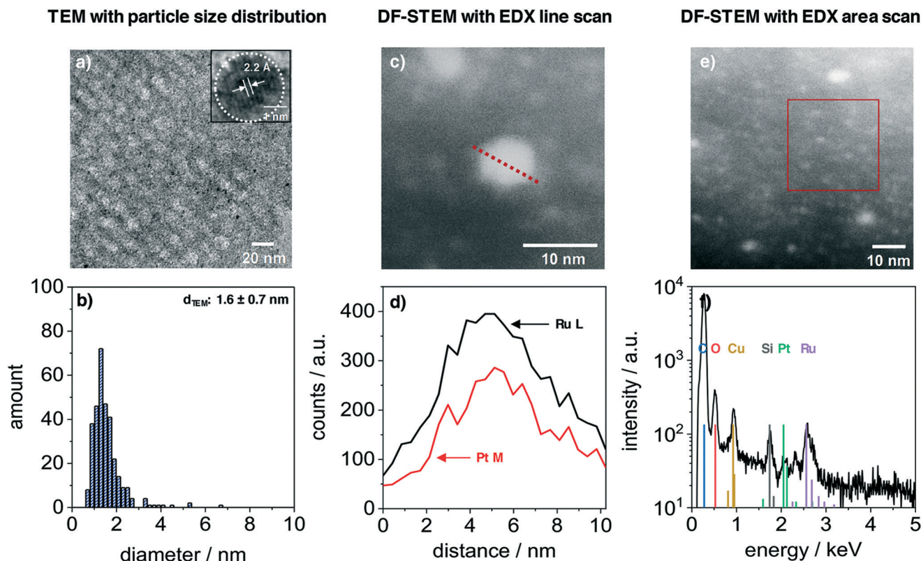
Fig. 3 TEM and STEM-EDX characterization of platinum-ruthenium nanoparticles (0.3 wt%Pt and 2.2 wt%Ru) in a mesoporous carbon film which was carbonized at 700 °C in H 2 /Ar, additionally heat-treated at 300 °C in air and reduced in H 2 /Ar at 350 °C. a) TEM image displays small nanoparticles throughout the film volume and a HR-TEM image (inset) indicates lattice planes of nanoparticles. The particles have an average diameter of 1.6 nm (b). c) Dark-field scanning TEM image with EDX line scan of a particle with a diameter of about 6 nm. d) Corresponding EDX analysis of the EDX line scans c). e) DF-STEM image with EDX area scan of smaller particles. f) Corresponding EDX analysis of the EDX area scan in e).
