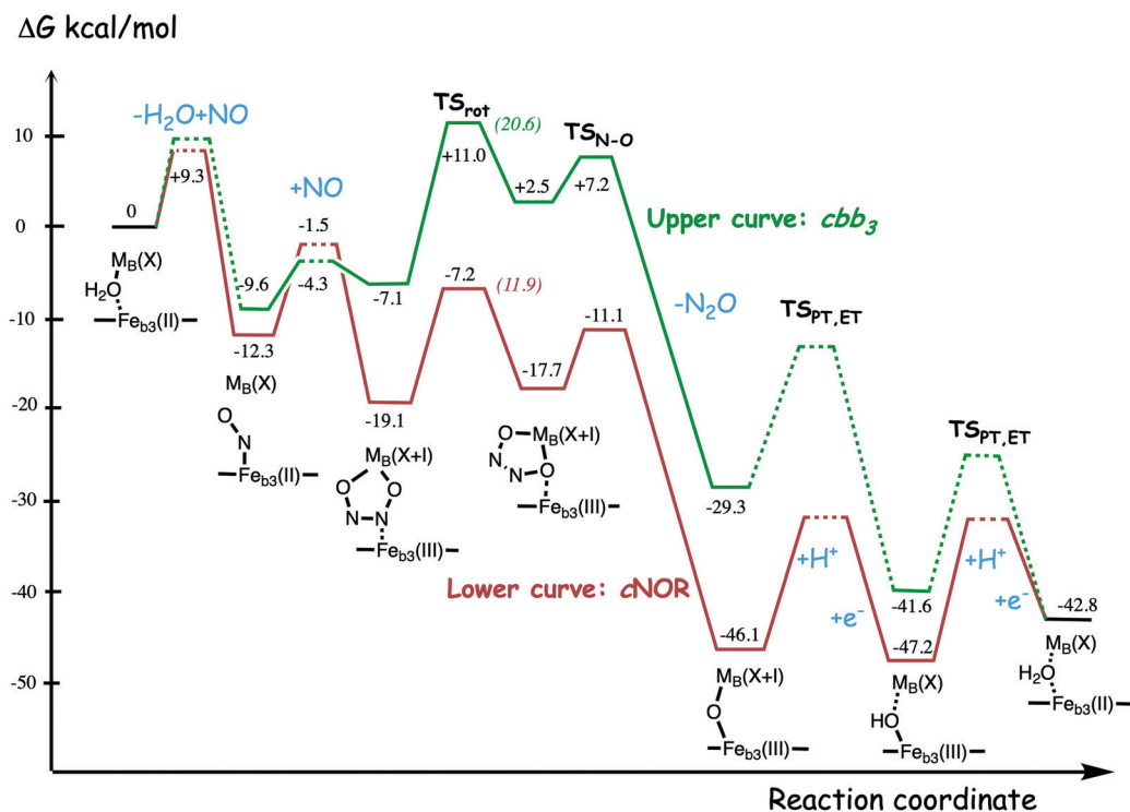
Fig. 24 Calculated free energy profile for one full catalytic cycle of NO reduction in cNOR 12 and in cbb 3 CcO using mechanism I. The notation M_B^{(X)} is used for Fe_B^{(ii)} in the cNOR case and for Cu_B^{(ii)} in the cbb 3 case, while the notation M_B^{(X+1)} is used for Fe_B^{(iii)} and Cu_B^{(iii)} , respectively. The dashed parts of the curves were not studied. The cNOR curve is here calculated relative to the ultimate electron donor cytochrome c , which is different from Fig. 20. The figure is reprinted with permission from ref. 125. Copyright (2020) American Chemical Society.
