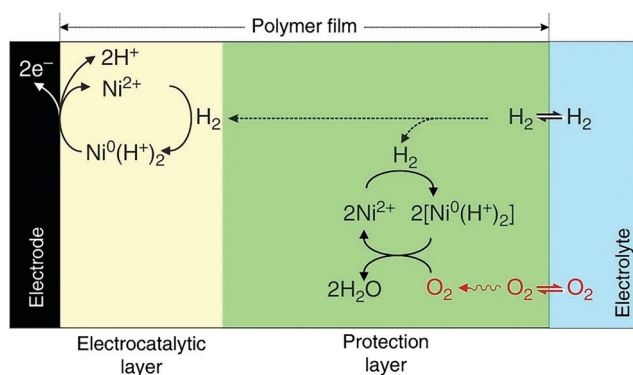
Fig. 13 A chemically inert polymer (PGMA-BA-PEGMA) is used to immobilize Dubois' Ni bis-diphosphine with glycine complex [\text{Ni}(\text{P}_2^{\text{Cy}}\text{N}_2^{\text{Gly}})_2]^{2+} on the surface of the electrode and prevent electrical contact between the metal complexes located within the polymer and the electrode. Two distinct regions are created: in the inner region (electrocatalytic layer), the Ni complex oxidizes \text{H}_2 , while in the outer region (protection layer), \text{Ni}^0 reduces \text{O}_2 to \text{H}_2\text{O} using the electrons produced from \text{H}_2 oxidation in the inner region. Reprinted with permission from ref. 280. (Creative Commons Attribution 4 International License).
