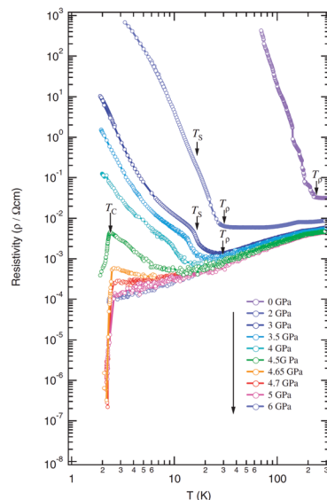
Fig. 16 Temperature dependence of resistivity of (\text{TMTTF})_2\text{AsF}_6 under various pressures, where T_p , T_s , and T_c are temperatures at minimum resistivity, spin-Peierls transition, and superconducting transition, respectively. Adapted with permission from ref. 72. Copyright 2007 Physical Society of Japan.
