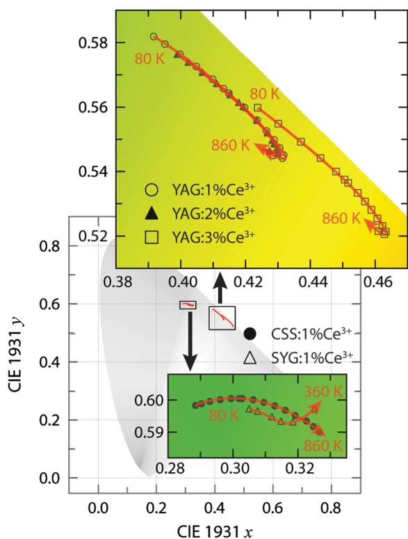
Fig. 3 Close-up views of the CIE 1931 color coordinate diagram for \text{YAG}:\text{z}\% \text{Ce}^{3+} ( z = 1, 2, and 3 ) in the green-yellow region, \text{CSS}:\text{1}\% \text{Ce}^{3+} , and \text{SYG}:\text{1}\% \text{Ce}^{3+} in the green region, upon excitation at 454\text{ nm} with varying temperature.
