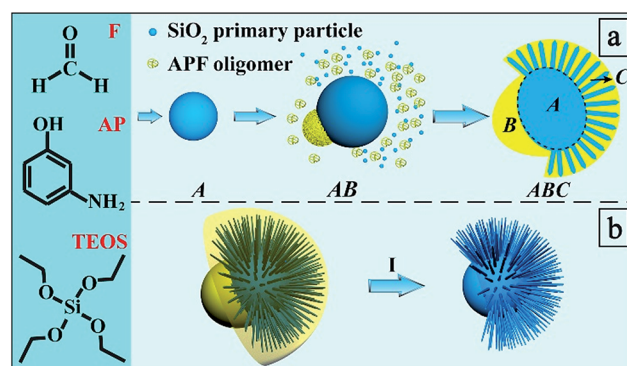
Scheme 1 Synthesis process and mechanism. (a) Bottom-up self-assembly of ABC type heterotrimeric nanoparticles and (b) their conversion into secondary Janus-type silica nanoparticles (I).
