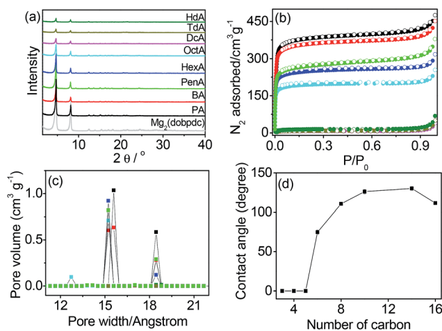
Fig. 1 (a) PXRD profiles, (b) N_2 isotherms at 77 K, and (c) pore size distributions of monoamine-appended Mg_2(\text{dobpdc}) . Color codes in (a)–(c) represent the same compounds. (d) Contact angles of the frameworks as a function of the number of carbons in the monoamine.
