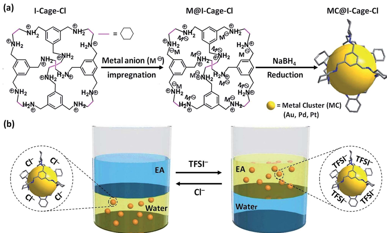
Scheme 1 (a) Synthetic scheme of MCs stabilized by I-Cage-Cl (Cl as counterion) in an aqueous phase (for clarity reasons \text{Cl}^- anions are omitted; \text{M}^\ominus = [\text{AuCl}_4]^- , [\text{PdCl}_4]^{2-} and [\text{PtCl}_4]^{2-} ). (b) Anion exchange-driven phase transfer of I-Cage-X ( \text{X} = \text{Cl}^- or \text{TFSI}^- , TFSI = bis(trifluoromethane sulfonyl)imide)-capped MCs between aqueous and ethyl acetate (EA) phases.
