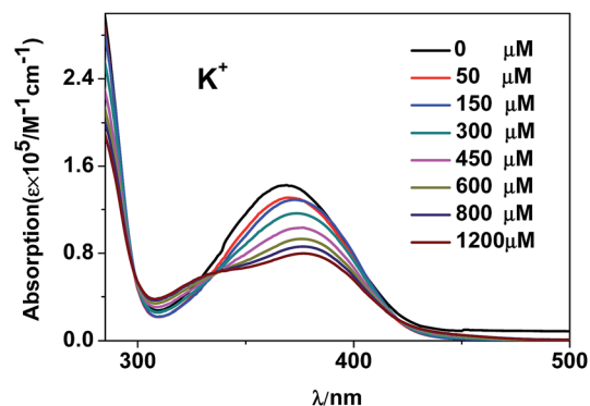
Fig. 9 UV-vis spectra of 1 ( 60 \mu M ) with the addition of K^+ ion.
