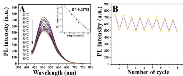
Fig. 5 (A) PL spectra of N-CDs obtained in the temperature range of 25\text{--}80^\circ\text{C} (inset: the emission intensity as a function of temperature). (B) Reversible fluorescence response of eight consecutive cycles from 25^\circ\text{C} to 80^\circ\text{C} .
