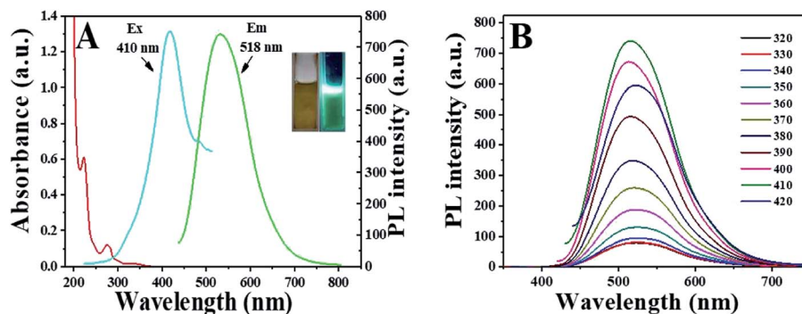
Fig. 4 (A) UV-vis absorption spectra, PL spectra of N-CDs obtained (insets are photographs of N-CDs obtained under visible and UV ( 365\text{ nm} ) light). (B) PL spectra of N-CDs obtained at different excitation wavelengths.
