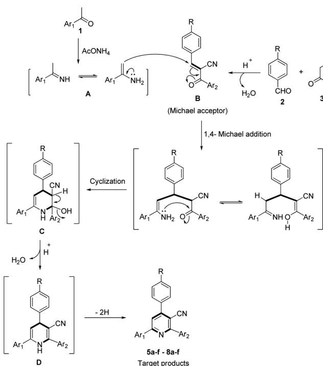
Scheme 3 A plausible mechanism pathway for the synthesized compounds 5a-f-8a-f .
