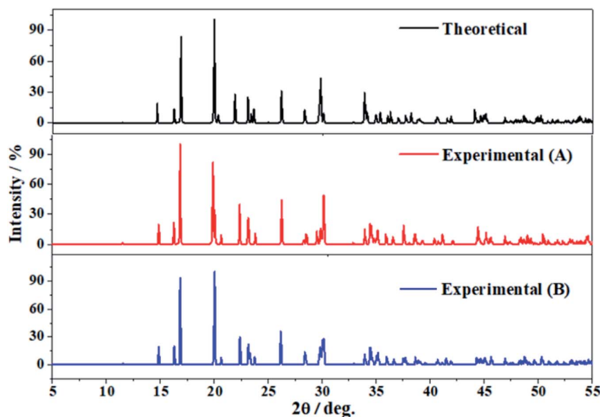
Fig. 3 X-ray diffraction powder patterns of vandenbrandeite using \text{CuK}\alpha radiation ( \lambda = 1.540598 \text{ \AA} ). The upper pattern has been determined from the calculated geometry. The mid pattern was obtained from the experimental geometry reported in this work. Finally the lower diffractogram is an experimental X-ray diffraction pattern from a natural sample from Shinkolobwe Mine, Shaba, Democratic Republic of Congo, taken from Record R080114 of RRUFF database. 183,184
