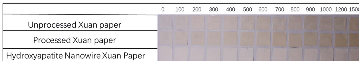
Fig. 7 Evaluation of the whiteness stability and durability of the as-prepared HNXp paper with a HAP/cellulose weight ratio of 35% by the accelerated heat aging method for up to 1500 years in comparison with the commercial Xuan paper: (a) whiteness; (b) tensile strength; (c) digital images of the three kinds of paper with increasing simulated aging time up to 1500 years.
