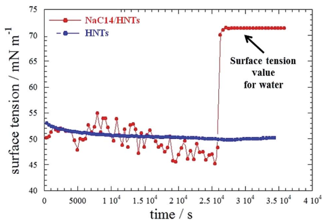
Fig. 8 Surface tension as a function of time for aqueous HNT and HNT/NaC14 dispersions in the presence of an n -decane film. Reproduced from ref. 38 with permission from the American Chemical Society, copyright 2014.
