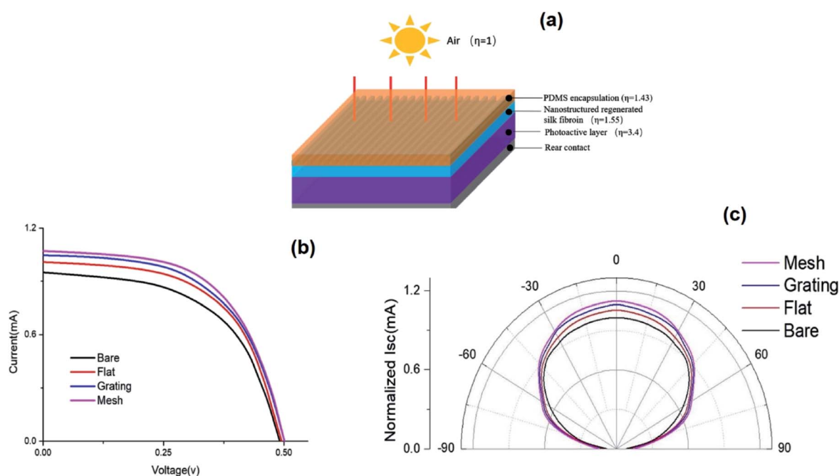
Fig. 7 (a) The schematics of the photodiode coated with the silk fibroin film; (b) The I-V curves of silicon photodiodes without (the black solid line) and with the encapsulated silk fibroin films; (c) the angular dependence of a normalized photocurrent without (the black solid line) and with encapsulated silk fibroin films, showing omnidirectional optical properties.
