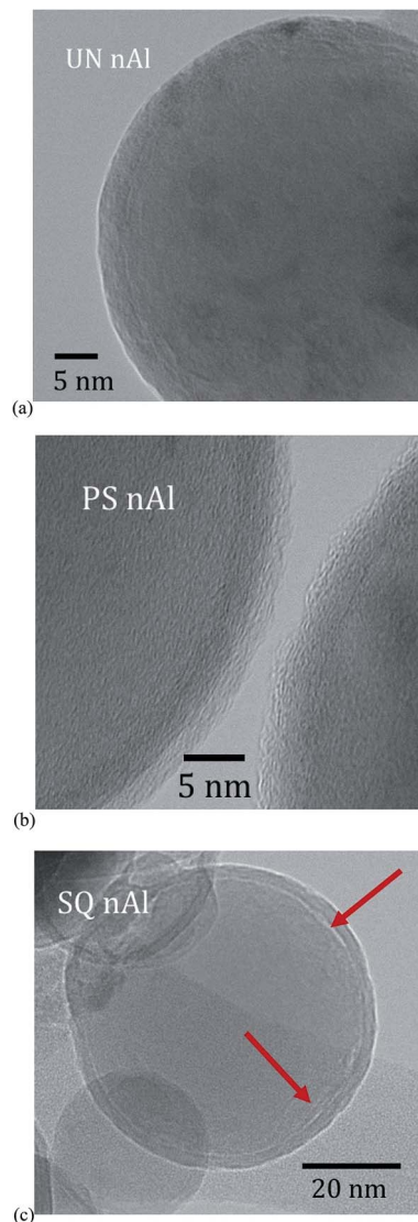
Fig. 4 TEM images of (a) UN nAl, (b) PS nAl, and (c) SQ nAl particles. Red arrows indicate regions of delamination.
