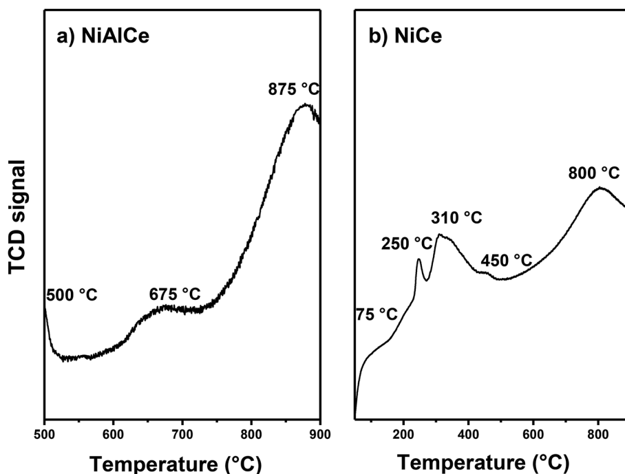
Fig. 12 \text{H}_2 -TPR profiles of calcined Ni NPS supported: (a) NiAlCe and (b) NiCe.
