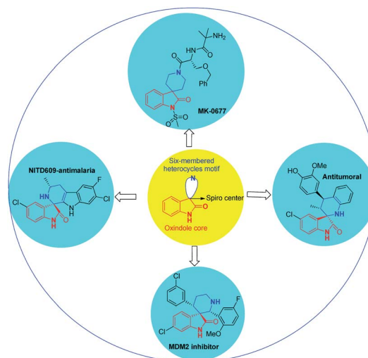
Fig. 1 Bioactive and medically important compounds containing a spiroimidazopyridineoxindole skeleton.
