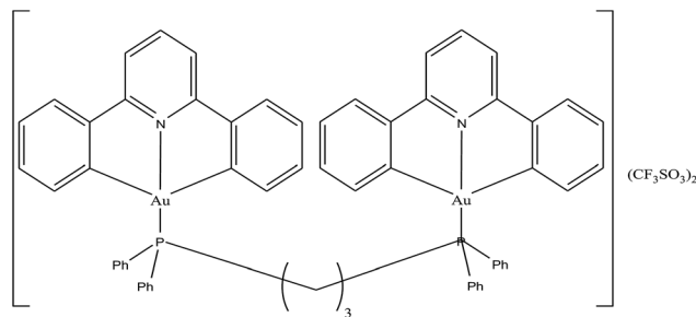
Fig. 27 Chemical structure of gold(III)-phosphine complex [Au_2(C^N^C)_2(\mu-dppp)](CF_3SO_3)_2 .
