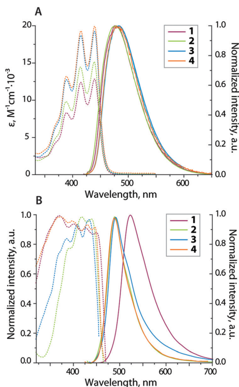
Fig. 5 (A) UV-vis absorption (dotted lines) and normalized emission (solid lines) spectra of 1–4 in \text{CH}_2\text{Cl}_2 (298 K, \lambda_{\text{ex}} = 415 \text{ nm} ); (B) normalized solid-state excitation (dotted lines) and emission (solid lines) spectra of 1–4 (298 K, \lambda_{\text{ex}} = 415 \text{ nm} ).
