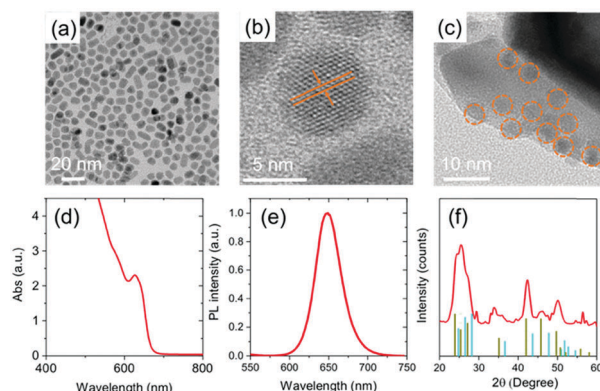
Fig. 3 TEM images: (a) (\text{CdSe})/(\text{CdSe}_x\text{S}_{1-x})_5/(\text{CdS})_1 heterostructured QDs; (b) HRTEM image; (c) HRTEM image of the QD sensitized \text{TiO}_2 mesoporous film, the dotted orange circles highlight the presence of QDs. Optical properties of QDs: (d) absorption spectrum in the UV-visible region of the as synthesized QDs in toluene; (e) PL spectrum of the QDs in toluene; (f) XRD pattern of the QDs. The Joint Committee on Powder Diffraction Standards (JCPDS) card files for CdSe (00190191, green dashed for ZB and 08-459, dark green for WZ) and CdS (01-077-2306, cyan for WZ) are shown for identification.
