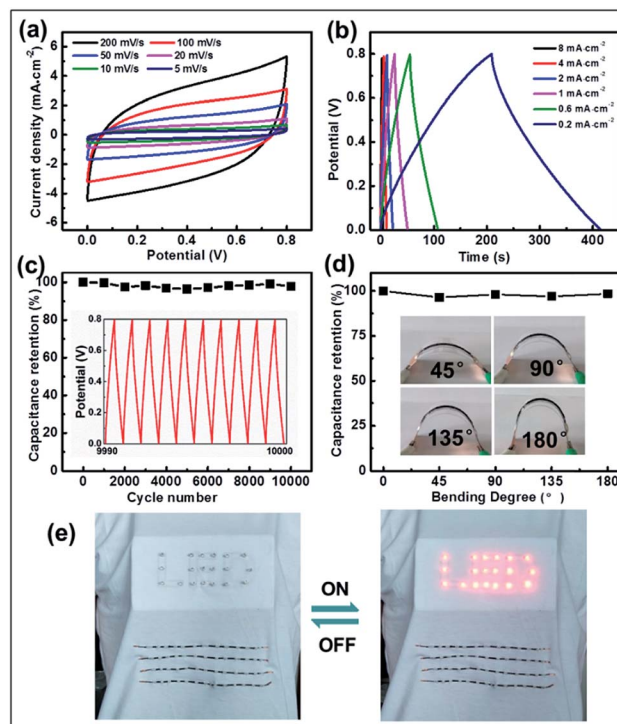
Fig. 5 (a) CV curves of micro-SCs based on CNB fibers in \text{H}_3\text{PO}_4 /PVA solid-state electrolyte, with scan rates increased from 5 to 10, 20, 50, 100 and 200 \text{mV s}^{-1} . (b) GCD curves of micro-SCs, with current density increased from 0.2 to 0.6, 1, 2, 4 and 8 \text{mA cm}^{-2} . (c) The cycling stability of micro-SCs at a voltage of 0.8 V at a current density of 0.4 \text{mA cm}^{-2} ; the inset: GCD curves after 10 000 cycles between 0 and 0.8 V. (d) Capacitance retention of the CNB micro-SCs at different bending states at a current density of 0.4 \text{mA cm}^{-2} . (e) Four CNB micro-SCs were connected in series into woven fabric and powered 19 LEDs.
