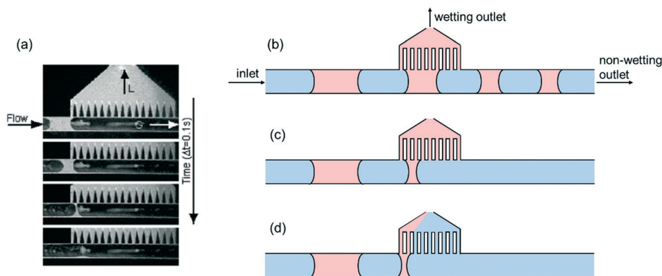
Fig. 1 (a) A series of photographs demonstrating the separation of a gas/liquid mixture using the capillary separator 22 (copyright 2005 by American Chemical Society); scheme of the different operation modes of the capillary separator when varying the pressure difference between the non-wetting and wetting outlets: (b) retention; (c) complete separation; (d) breakthrough.
