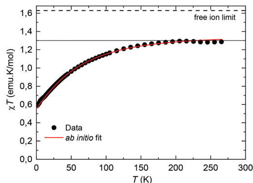
Fig. 4 Temperature dependence of \chi T for complex (1). The dotted line marks the predicted \chi T (300 K) value for a Nd(III) free ion with gyromagnetic value g_J = 0.727 . 40 Red line: fit within a chain model of Nd ions, with ab initio calculated wavefunctions and intrachain interaction J'/k_B = -3.15 \times 10^{-3} K.
