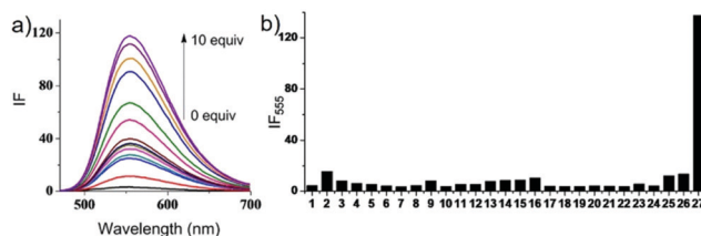
Fig. 85 (a) Fluorescent emission spectra of 10 \mu M probe 55 in the presence of 0–10 equiv. of H_2S in aqueous solution ( CH_3CN/PBS = 1:9 , pH = 7.4, 37 ^{\circ}C ) (NaHS was dissolved in water at a concentration of 10 mM). Excitation at 450 nm. (b) Fluorescence responses of 10 \mu M 55 to various analytes in aqueous solution ( CH_3CN/PBS = 1:9 , pH = 7.4, 37 ^{\circ}C ). Excitation at 450 nm. Bars represent the final fluorescence intensity of 55 with 1 mM analytes over the original emission of free 55 . (1) Free 55 ; (2) Zn^{2+} ; (3) Na^+ ; (4) Ca^{2+} ; (5) K^+ ; (6) Mg^{2+} ; (7) HCO_3^- ; (8) F^- ; (9) Cl^- ; (10) Br^- ; (11) I^- ; (12) NO_3^- ; (13) S_2O_3^{2-} ; (14) S_2O_4^{2-} ; (15) S_2O_5^{2-} ; (16) SO_3^- ; (17) N_3^- ; (18) CO_3^{2-} ; (19) CH_3COO^- ; (20) SO_4^{2-} ; (21) H_2O_2 ; (22) HSO_4^- ; (23) homocysteine; (24) ascorbic acid; (25) cysteine; (26) glutathione; and (27) NaHS. Copyright 2013 American Chemical Society.
