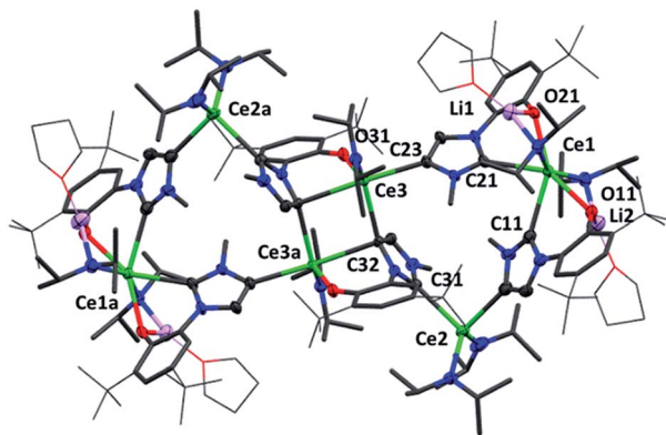
Fig. 4 Molecular structure of 5\text{Ce}^{\text{Me}} with imidazolium, Ce, O and Li atoms shown at 50% ellipsoid probability, framework atoms drawn capped stick and coordinated solvents, peripheral carbon atoms wireframe, and H and lattice solvent omitted for clarity. Selected distances (Å) and angles ( ^{\circ} ) for 5\text{Ce}^{\text{Me}} : Ce1–C11 2.743(5), Ce1–C21 2.728(5), Ce2–C13 2.667(7), Ce2–Ce31 2.710(5), Ce3–C23 2.651(6), Ce3–C32 2.854(4), Ce3–C32a 2.685(6), Ce1–O11 2.517(4), Ce1–C21 2.462(4), Ce3–O31 2.232(3), C11–Ce1–O11 65.1(2), C11–Ce1–C21 82.1(2), C21–Ce1–O21 65.9(1), C13–Ce2–C31 94.4(2), Ce3–C32–Ce3a 98.5(1), C32–Ce3–C32a 81.5(1), C32–Ce3–O31 71.1(1), C32–Ce3–C32a 163.8(2).
