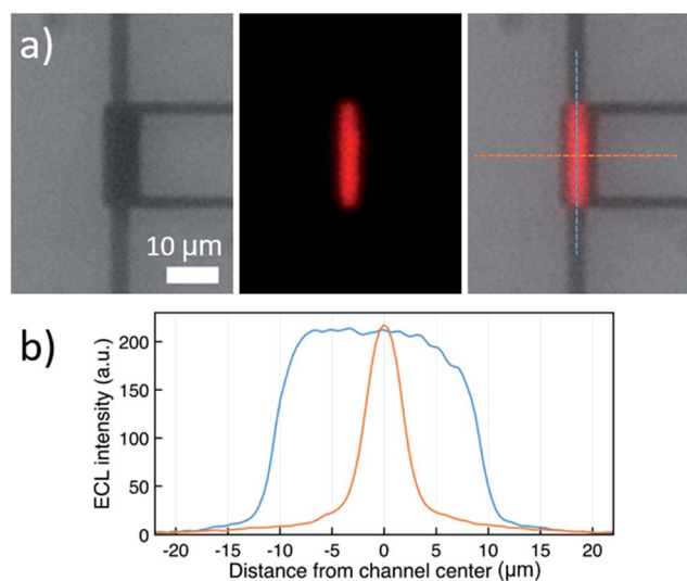
Fig. 3 (a) From left to right: bright-field micrograph of the nano-channel, ECL emission recorded in the dark, and overlay of both images (dashed lines: direction of profiles in (b)). (b) ECL intensity profiles along (blue) and across (orange) the center of the channel, using a solution of 10 mM Ru(bpy) 3 (PF 6 ) 2 and 0.1 M TBAPF 6 in acetonitrile. The top electrode was biased at 2 V, the bottom electrode at -1.5 V vs. Ag.
