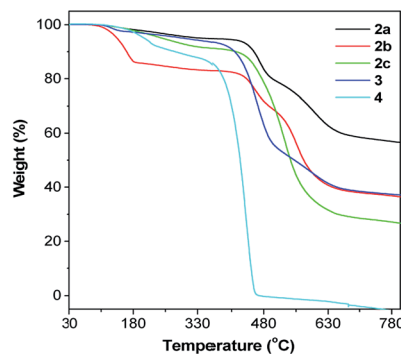
Fig. 1 TGA curves of TPE-Pys recorded under nitrogen at a heating rate of 10 °C min -1 .
