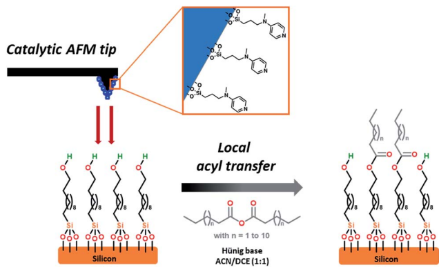
Fig. 1 Schematic representation of the interface between the SAM-coated substrate and the AFM catalytic tip.
