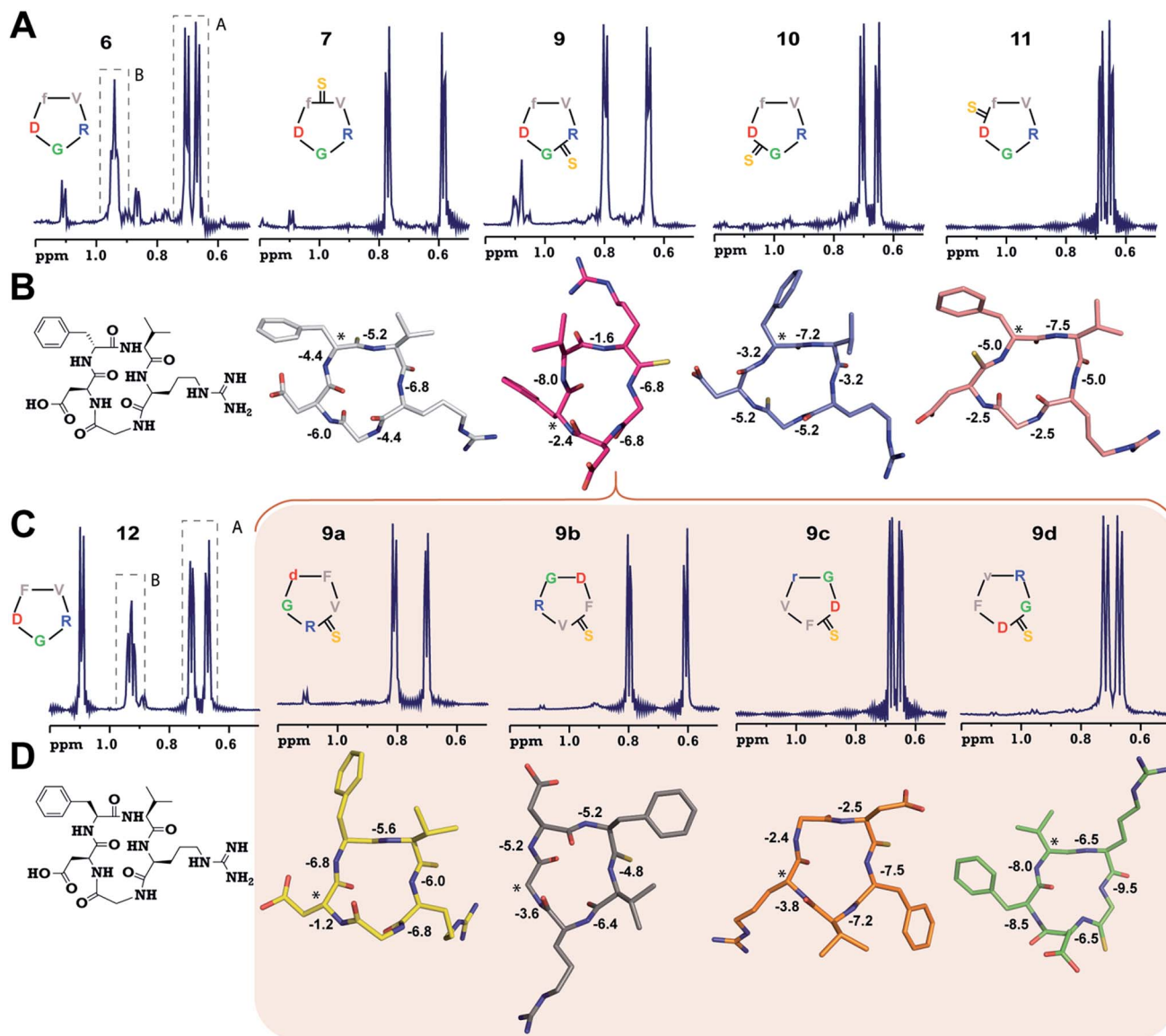
Fig. 2 (A) 1 H NMR spectra of cyclo(RGDfV) (6) and its thio-analogs 7–11. The γ-CH 3 of Val in both the conformers (A and B) of 6 is shown. (B) The solution structures of 7–11 deduced from 2D 1 H NMR spectroscopy in aqueous conditions. (C) 1 H NMR spectra of cyclo(RGDfV) (12) showing two conformers. (D) Solution structures of spatial screen analogs of 9 (9a–9d). The temperature coefficients of the amide protons (ppb K -1 ) are shown and the asterisk denotes the site of the D-amino acid (Gly in 9b). Significant resonance overlap precluded the structure determination of 6 and 12. The hydrogen atoms are omitted for the sake of clarity.
