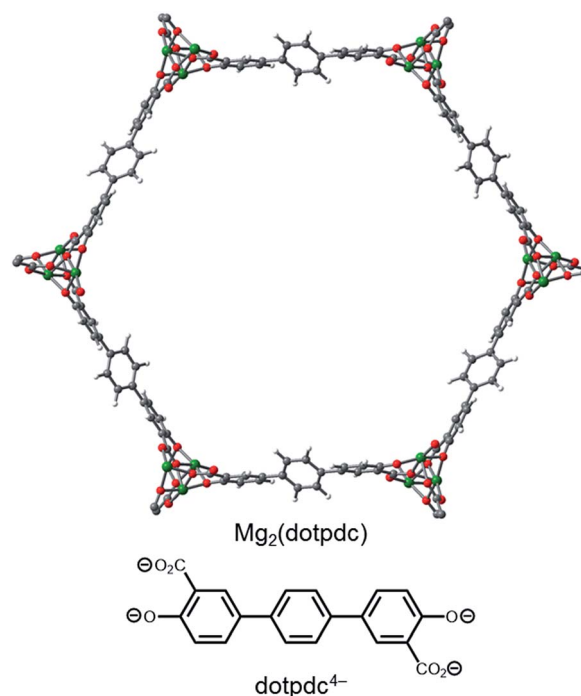
Fig. 7 Structure of the organic linker \text{dotpdc}^{4-} = 4,4'' -dioxido-[1,1':4',1''-terphenyl]-3,3''-dicarboxylate and a model of the hexagonal pore of \text{Mg}_2(\text{dotpdc}) . Green, grey, red, and white spheres correspond to Mg, C, O, and H, respectively.
