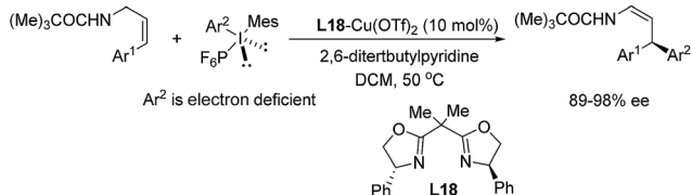
Scheme 14 Cu/BOX-catalyzed enantioselective electrophilic arylation of allylic amides.
