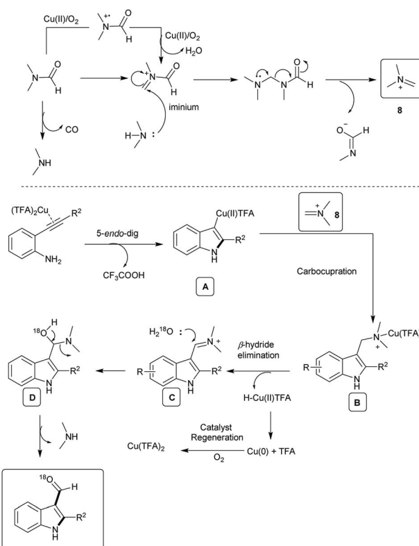
Scheme 6 Proposed mechanism.
