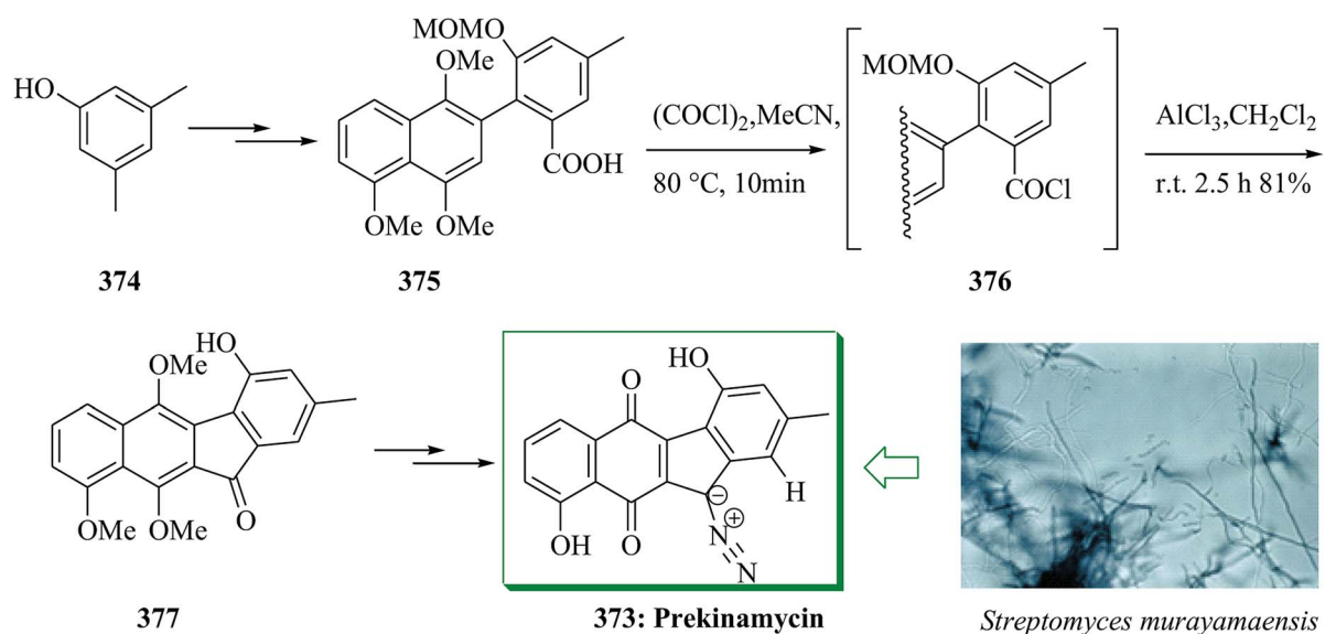
Scheme 79 Total synthesis of prekinamycin 373.
