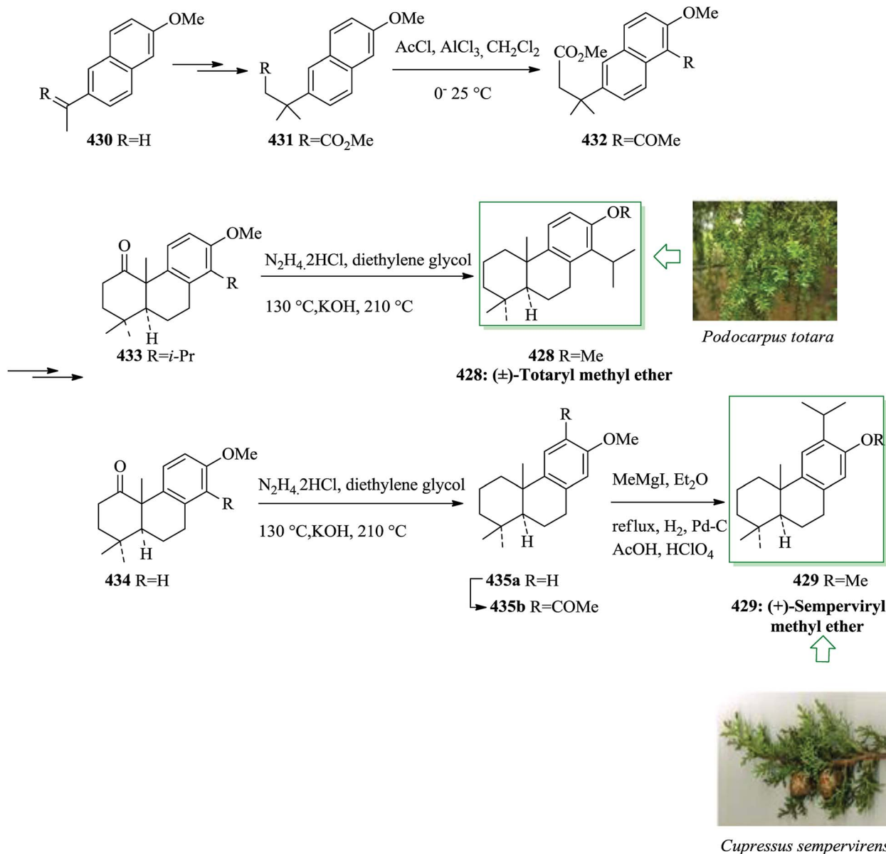
Scheme 91 Total synthesis of ( \pm )-totaryl methyl ether 428 and (+)-semperviryl methyl ether 429.
